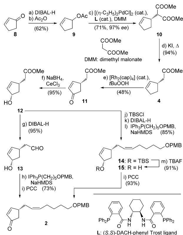
Scheme 1. Synthesis of cyclopentenone fragment 2 . Reagents and conditions: a) DIBAL-H (1 M in CH 2 Cl 2 , 1.2 equiv), CH 2 Cl 2 , 0 °C, 30 min; b) Ac 2 O (2.0 equiv), Et 3 N (2.5 equiv), DMAP (0.1 equiv), CH 2 Cl 2 , 0→25 °C, 18 h, 62 % for two steps; c) dimethyl malonate (3.0 equiv), [\eta^3\text{-C}_3\text{H}_5\text{PdCl}]_2 (0.005 equiv), ( S,S )-DACH-phenyl Trost ligand (0.015 equiv), Cs 2 CO 3 (3.0 equiv), CH 2 Cl 2 , 25 °C, 3 h, 71 %; d) KI (8.0 equiv), DMI/H 2 O (10:1), 130 °C, 12 h, 94 %; e) [Rh 2 (cap) 4 ] (0.01 equiv), t BuOOH (5.0 equiv), K 2 CO 3 (0.5 equiv), CH 2 Cl 2 , 1.5 h, 25 °C; then [Rh 2 (cap) 4 ] (0.01 equiv), t BuOOH (5.0 equiv), 1.5 h, 25 °C, 48 %; f) CeCl 3 ·7H 2 O (1.0 equiv), NaBH 4 (1.0 equiv), −30 °C, 10 min, 95 %; g) DIBAL-H (1 M in CH 2 Cl 2 , 2.2 equiv), CH 2 Cl 2 , −78 °C, 45 min, 95 %; h) IPH 3 P(CH 2 ) 5 OPMB (2.5 equiv), NaHMDS (1 M in THF, 3.0 equiv), THF, −78→25 °C, 18 h, 79 %; i) PCC (2.0 equiv), CH 2 Cl 2 , 25 °C, 3 h, 93 %; j) TBSCl (1.5 equiv), imid. (3.0 equiv), CH 2 Cl 2 , 0→25 °C, 15 min; k) DIBAL-H (1 M in CH 2 Cl 2 , 1.1 equiv), CH 2 Cl 2 , −78 °C, 45 min; l) IPH 3 P(CH 2 ) 5 OPMB (1.5 equiv), NaHMDS (1 M in THF, 2.0 equiv), THF, −78→25 °C, 6 h, 85 % for three steps; m) TBAF (1 M in THF, 1.2 equiv), THF, 0→25 °C, 5 h, 91 %. DACH-phenyl Trost ligand = 1,2-diaminocyclohexane- N,N' -bis(2'-diphenylphosphinobenzoyl); DIBAL-H = diisobutylaluminum hydride; DMAP = 4-dimethylaminopyridine; DMI = 1,3-dimethyl-2-imidazolidinone; DMM = dimethyl malonate; imid. = imidazole; NaHMDS = sodium bis(trimethylsilyl)amide; PCC = pyridinium chlorochromate; PMB = para -methoxybenzyl; [Rh 2 (cap) 4 ] = dirhodium tetracaprolactamate; TBAF = tetrabutylammonium fluoride; TBS = tert -butyldimethylsilyl; THF = tetrahydrofuran.
